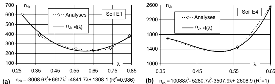
Fig. 9. Relation of the parameters n_{ck} and \lambda to polynomial functions for small values of \lambda .
